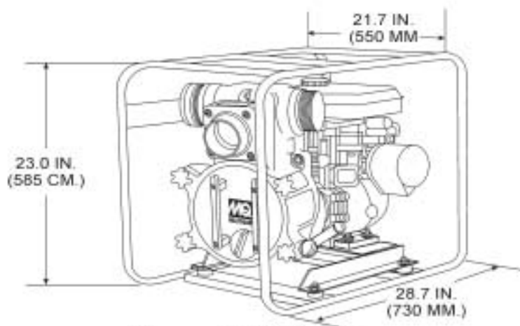
Figure1. QP-3TH Dimensions
