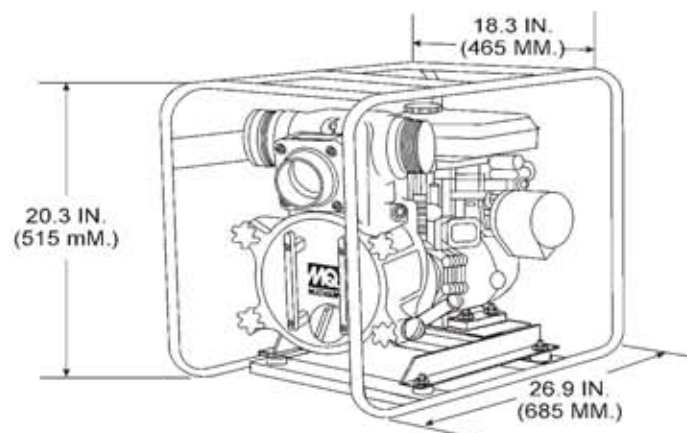
Figure 1. QP-2TH Dimensions
